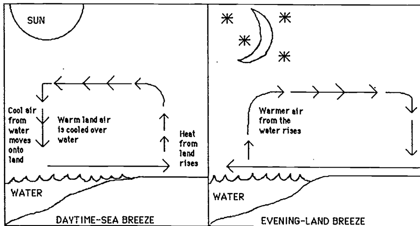
Weather fronts bring rapid changes in wind and weather conditions. Most notable are "cold fronts" that usher in rapid changes in air temperatures and turbulent winds. The figure above shows how surface waters and day and night-time temperatures affect winds or breezes. (Courtesy of National Oceanic and Atmospheric Administration).
